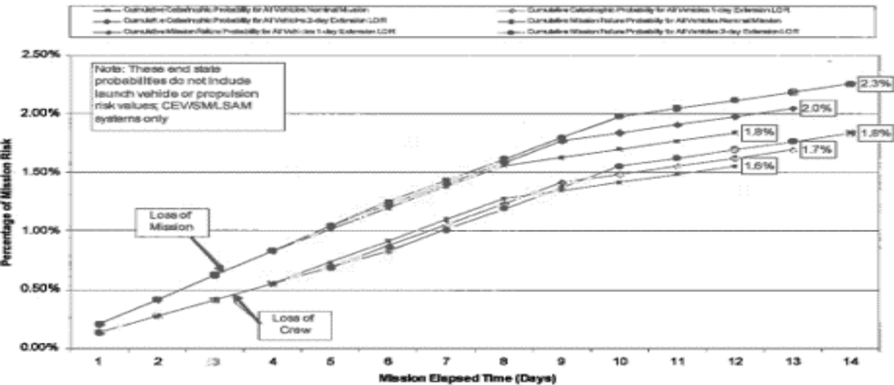
Figure 1 - Pre-landing loiter in lunar orbit
